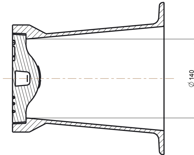
REZ B - B section B - B
