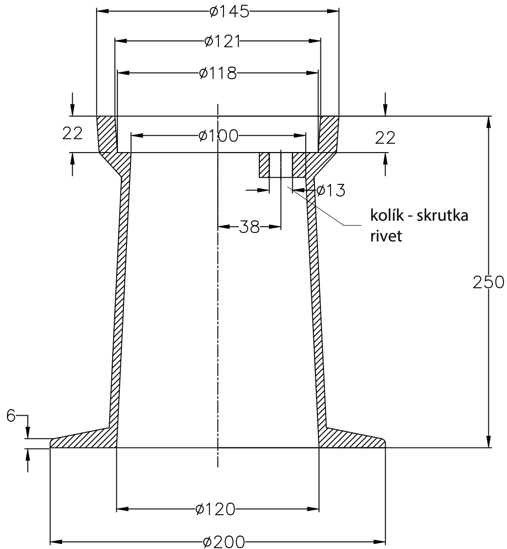
REZ A - A section A - A
